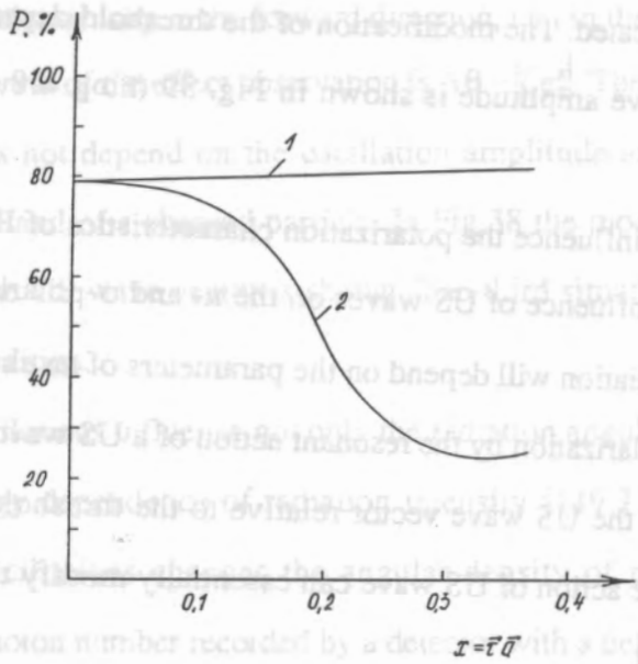
Fig. 40. Here: P is the PXR polarization power in Si (220), \theta_D = 10^{-3} rad, \alpha = z\alpha_{th} : 1) z = 1 , v_s = 4.17 \cdot 10^8 Gz; 2) z = 1.5 , v_s = 6.26 \cdot 10^8 Gz.
