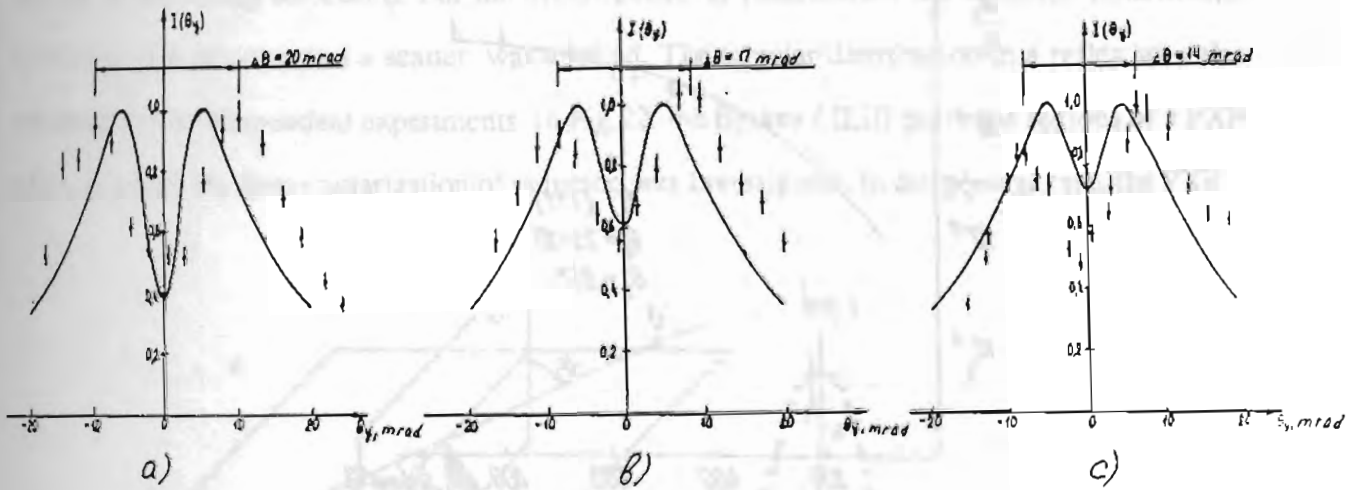
Fig. 20. The vertical PXR angular distribution: a) E = 900 MeV; b) E = 500 MeV; c) E = 370 MeV.
