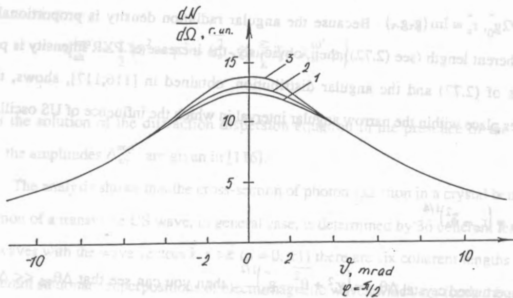
Fig. 36. Here: L = 2 \text{ mm} , \alpha = \alpha_{th} , the US frequency \nu \cong 7.54 \cdot 10^8 \text{ Gz} , g = 1/2 \tau a are 1) 0; 2) 0.06; 3) 0.1.
