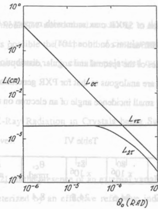
Fig. 34. Here: L_{0\tau} is the vacuum coherent length, L_{1\tau} and L_{2\tau} are the coherent lengths inside the medium, \theta_0 is the beam particle incidence angle.
