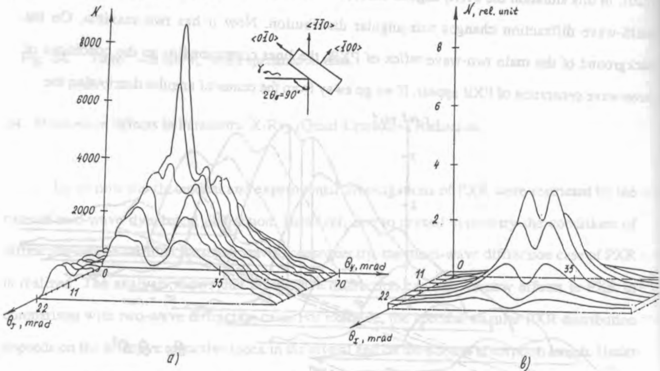
Fig. 26. Here: a) the experimental distribution under multi-wave diffraction; b) the theoretical distribution for (400) reflex under two-wave diffraction.
